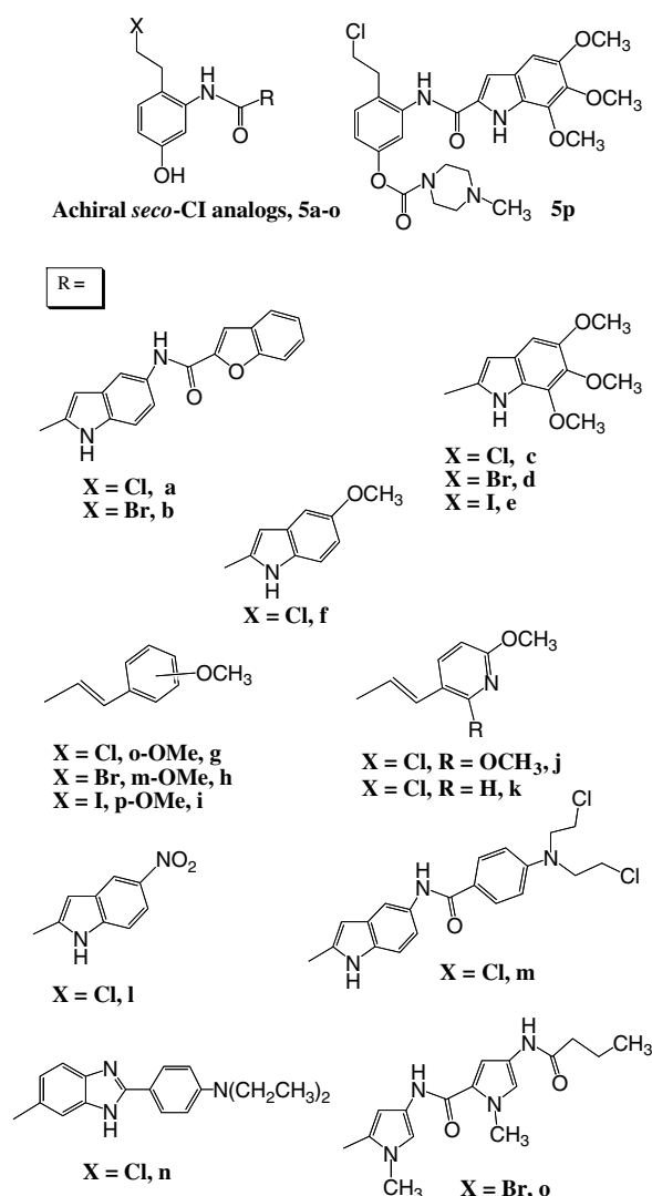
Figure 3. Fifteen analogs of achiral seco -CI prepared in this study, 5a–o , and a carbamate derivative 5p .
