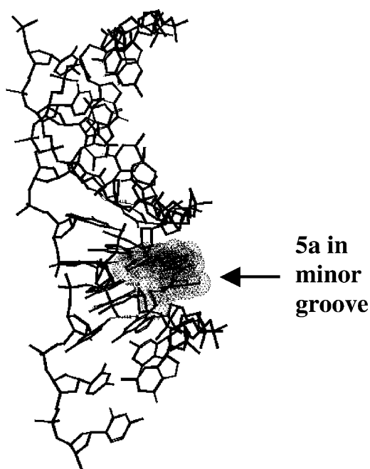
Figure 6. MM2 energy optimized (steepest descend) structure of a complex of a covalent adduct between the chloromethyl moiety of compound 5a and adenine-N3 of the underlined residue of duplex dGGCGGAGTTAAGG in the B-form.
