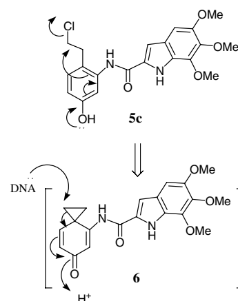
Figure 2. Proposed mechanism of activation and DNA alkylation of the achiral seco -CI moiety in compound 5.
