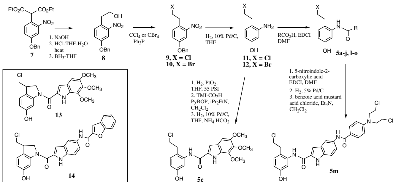
Scheme 1. Synthesis of the achiral seco -CI analogs of CC-1065 and the duocarmycins.
