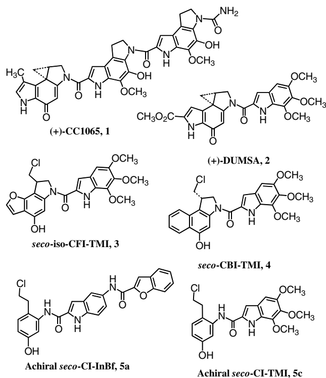
Figure 1. Structures of (+)-CC-1065 (1), (+)-duocarmycin SA (DUMSA, or 2), seco -iso-CFI-TMI (3), and seco -CBI-TMI (4).
